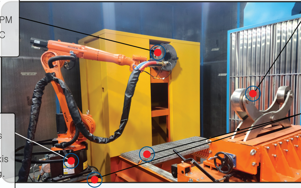
6 Axes Robot with 7 th Axis Liner Track
